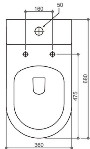
TOP VIEW
