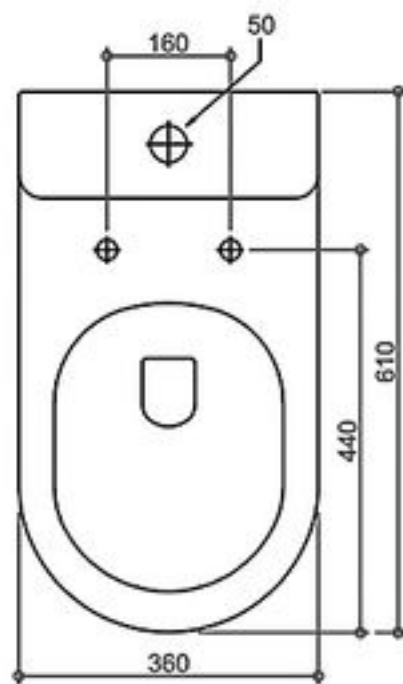
TOP VIEW
