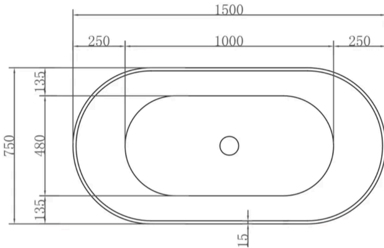
Top View
