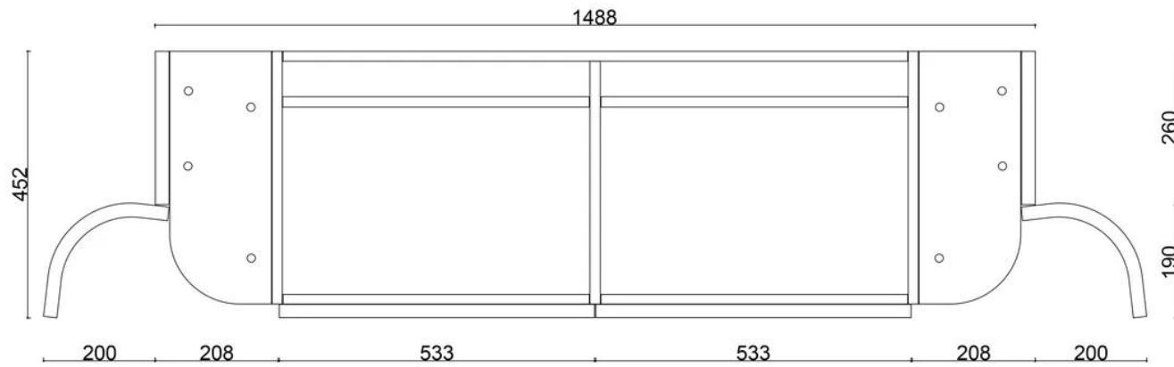
TOP VIEW
