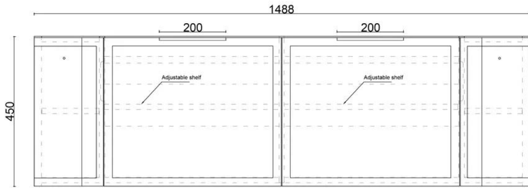
FRONT VIEW
