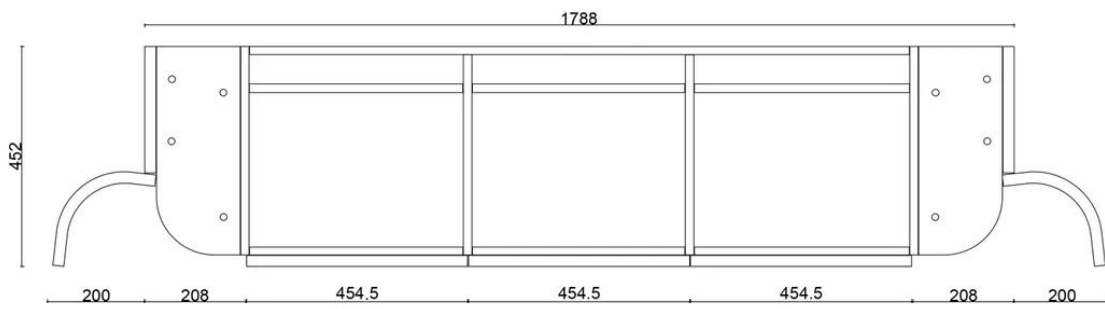
TOP VIEW
